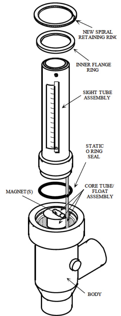
Fig. 1: Partially exploded drawing of the MEMFlo All Metal Flow Meter
